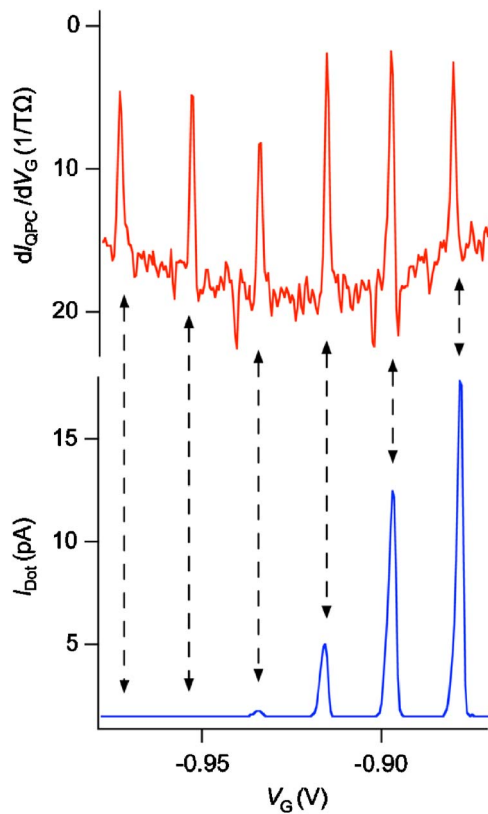
FIG. 2. (Color online) (top) The derivative of the quantum point contact current with respect to the gate voltage dI_{QPC}/dV_G as a function of the gate voltage V_G . The peaks correspond to changes in the number of electrons in the dot. (bottom) The current through the quantum dot as a function of the gate voltage V_G . The peaks in the two curves are well aligned, indicating that the charge-sensing quantum point contact and the Coulomb blockade peaks in transport through the dot correspond to the same quantum dot charging phenomena.
