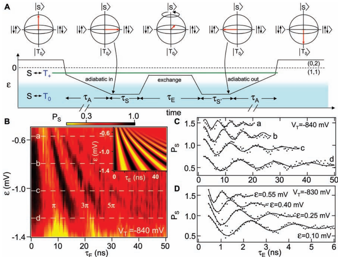
Fig. 4. (A) Pulse sequence demonstrating exchange control. After initializing into (0,2)S , detuning \epsilon is swept adiabatically with respect to tunnel coupling through the S-T_+ resonance (quickly relative to S-T_+ mixing), followed by a slow ramp ( \tau_A \sim 1 \mu\text{s} ) to large detuning, loading the system in the ground state of the nuclear fields |\uparrow\downarrow\rangle . An exchange pulse of duration \tau_E rotates the system about the z axis in the Bloch sphere from |\uparrow\downarrow\rangle to |\downarrow\uparrow\rangle . Reversing the slow adiabatic passage allows the projection onto (0,2)S to distinguish states |\uparrow\downarrow\rangle and |\downarrow\uparrow\rangle after time \tau_E . Typically, \tau_S = \tau_{S'} = 50 ns. (B) P_S as a function of detuning and \tau_E . The z -axis rotation angle \phi = J(\epsilon)\tau_E/\hbar results
