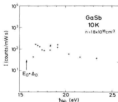
FIG. 6. Total intensity I ( = I_+ + I_- or I_{||} + I_{\perp} ) of the E_0 + \Delta_0 luminescence in GaSb as a function of the laser energy \hbar\omega_L . The intensity has been normalized with respect to the incident power.
