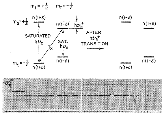
FIG. 4. Illustration of the method used to determine T_x in the presence of a much shorter T_s in phosphorus doped silicon ( 7 \times 10^{16} P/cm 3 , T = 1.25^\circ\text{K} , H \approx 3200 oersteds, Sample: Si VIII-64). From the amplitudes of the lines and the time interval during which T_x was operative one obtains at 3200 oersteds a value of T_s \approx 30 hours. Note that the saturation procedure results in a normal Overhauser effect and gives rise to the predicted nuclear polarization.
