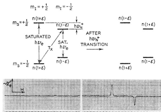
FIG. 4. Illustration of the method used to determine T_x in the presence of a much shorter T_s in phosphorus doped silicon ( 7 \times 10^{15} P/cm 3 , T = 1.25^\circ\text{K} , H \approx 3200 oersteds, Sample: Si VIII-64). From the amplitudes of the lines and the time interval during which T_x was operative one obtains at 3200 oersteds a value of T_x \approx 30 hours. Note that the saturation procedure results in a normal Overhauser effect and gives rise to the predicted nuclear polarization.
