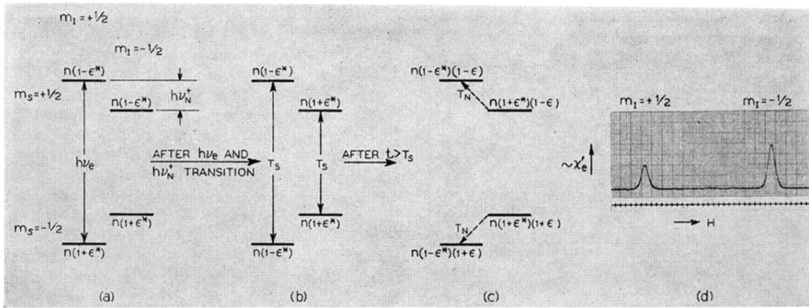
FIG. 5. Illustration of the method used to determine T_N in the presence of a shorter T_s (but longer T_2 ) in phosphorus doped silicon; (a) The magnetization is brought to thermal equilibrium at a high field. The corresponding Boltzmann factor is 2\epsilon^* ; (b) After a double adiabatic fast passage the m_I levels are preferentially occupied; (c) The populations after t > T_s ; (d) The experimental trace from phosphorus doped silicon ( 7 \times 10^{16} P/cm 3 , T = 1.25^\circ\text{K} , H = 3200 oersteds). The expected ratio of amplitudes is \sim (1+\epsilon^*)/(1-\epsilon^*) . From the rate at which the amplitudes of the two lines tend to equalize T_N may be obtained. Note the large nuclear polarization that is obtained during this procedure.
