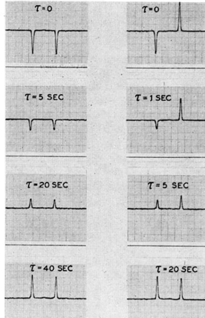
FIG. 8. The T_s and T_{ss} mechanisms in phosphorus doped silicon with \approx 4 \times 10^{16} conduction electrons/cm 3 introduced by light ( 0.5 \text{ eV} < h\nu < 0.66 \text{ eV} ). When both lines are inverted by an adiabatic fast passage only the T_s mechanism is effective. With only one line inverted the T_{ss} mechanism is seen to be predominant. From the above traces one finds that T_s \approx 25 sec. T_{ss} \approx 1 sec. The large difference between T_s and T_{ss} indicates the polarization of conduction electrons by exchange scattering ( T = 1.23^\circ \text{K} , \sim 7 \times 10^{15} \text{ P/cm}^3 , H \approx 3200 oersteds).
