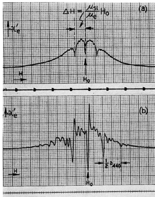
FIG. 11. "Discrete" spin diffusion in As -doped silicon ( \sim 2 \times 10^{16} As /cm 3 , T = 1.3^\circ\text{K} , H \approx 3200 oersteds). The line was saturated by setting H = H_0 and then turning the microwave power on. ( H_1 \approx 10^{-2} oersteds for \approx 10 sec.) The notches are displaced from H_0 by amounts corresponding to the Larmor frequencies of the \text{Si}^{29} nuclei at the different lattice points; (a) Direct detection without field modulation. (b) With magnetic field modulation.
