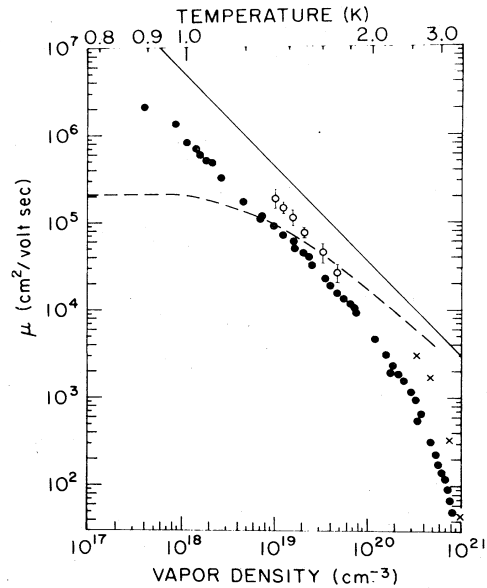
FIG. 8. The temperature-dependent mobility of an external surface state electron moving parallel to the surface. The theory (dashed line) includes both ripplon and gas atom scattering (Co70b). Open circles are data of (BG72); solid circles from (ST71). The solid line and crosses are theory and experiment, respectively, in three-dimensional vapor (M46, LS67).
