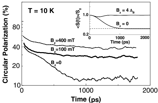
FIG. 3. Circular polarization dynamics of the QD ground state luminescence (semilogarithmic scale) for B_z = 0 , B_z = 100 mT, and B_z = 400 mT. The inset displays the calculated time dependence of the average electron spin \langle S(t) \rangle / S_0 (see text).
