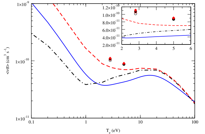
FIG. 3 (color online). The radiative recombination rate coefficient as a function of the electron temperature. The lines only use positive energy states: the solid (blue) line is from experiment [10], the dashed (red) line is from the AUTOSTRUCTURE calculation described in the text, the dash-dotted (black) line is when the positive energy states below 70 meV are shifted to just below threshold. The symbols include the negative energy states. Open symbols are for 10^4 \text{cm}^{-3} and closed symbols are for 10^8 \text{cm}^{-3} . The diamonds are for the correct AUTOSTRUCTURE calculation and the circles are when the positive energy states below 70 meV are shifted to just below threshold. Because the data for negative energy states varies little, some of the symbols are not clearly visible.
