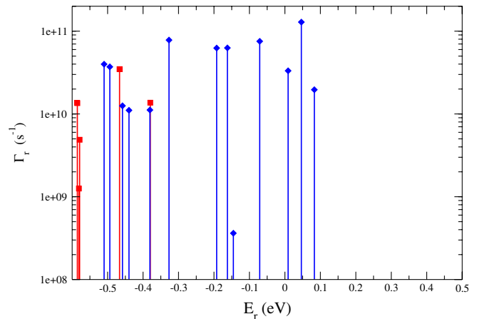
FIG. 1 (color online). The temperature-independent contribution of the Mg^{7+} states to the DR rate coefficient, \Gamma_r \equiv (2J_r + 1)/[2(2J_c + 1)][\Gamma_R \Gamma_A / (\Gamma_R + \Gamma_A)] , as a function of energy, E_r , relative to the ionization threshold. The energies were obtained from the AUTOSTRUCTURE program shifting the core energies to the NIST values. The squares show the resonances belonging to the 2s2p(^3P)7p configuration and the diamonds show the resonances belonging to the 2s2p(^3P)7d configuration. Resonances belonging to the 2s2p(^3P)7\ell configuration with \ell \geq 3 are also in this energy range but have a negligible strength.
