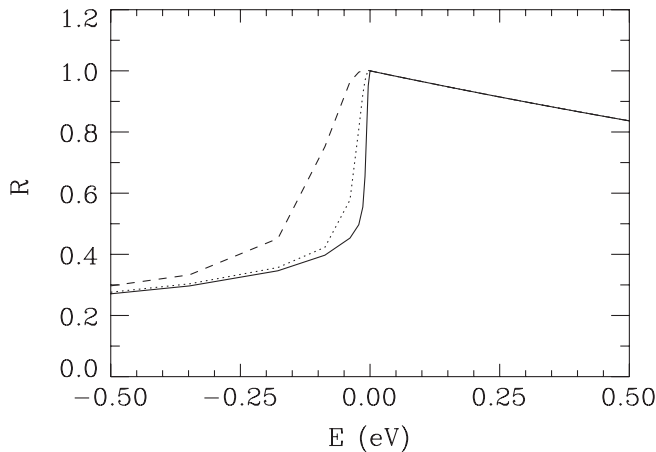
FIG. 2. The \text{Mg}^{7+} relative population R = \exp(-E/T)\xi(E) for negative energy and, R = \exp(-E/T) at positive energy for an electron temperature of 2.8 eV. The solid line is for a density of 10^4 \text{ cm}^{-3} , the dashed line is for 10^6 \text{ cm}^{-3} , and the dot-dashed line is for 10^8 \text{ cm}^{-3} . The population smoothly extends to negative energy, but has an initial decrease at negative energy which becomes sharper with decreasing density. The 1s^2 2s^2 n\ell Rydberg populations were calculated using the ADAS204 code [17]. In this calculation, the DR rate coefficients were taken from Ref. [19] and the rest of the radiative and collisional rates were taken from semiclassical expressions.
