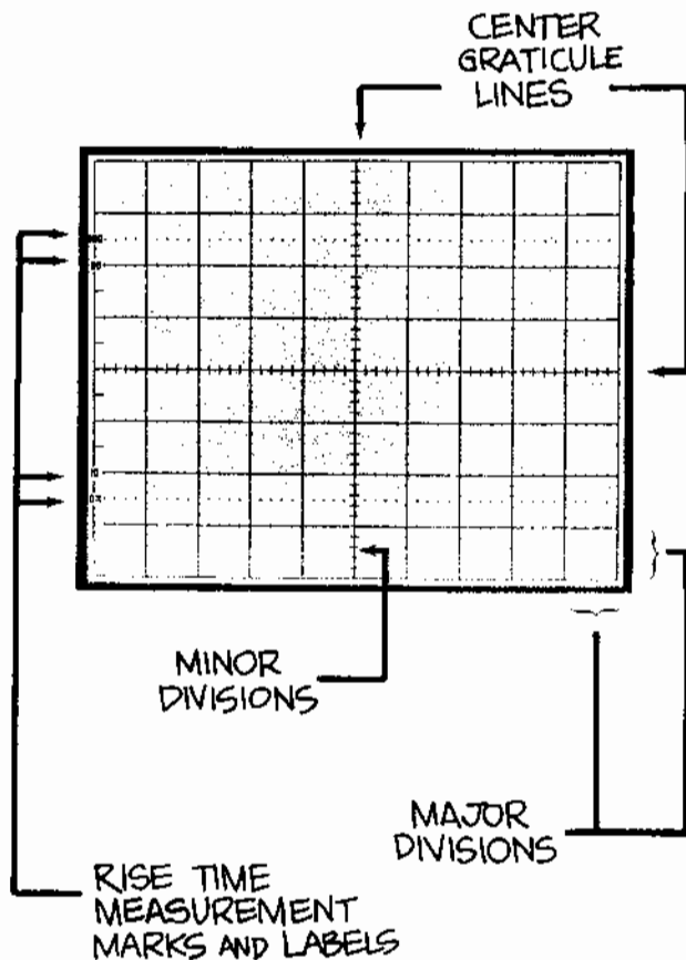
Figure 2. THE GRATICULE is a grid of lines typically etched or silk-screened on the inside of the CRT faceplate. Putting the graticule inside — or the same plane as the trace drawn by the electron beam — and not on the outside of the glass — eliminates measurement inaccuracies called parallax errors . Parallax errors occur when the trace and the graticule are on different planes and the observer is shifted slightly from the direct line of sight. Though different sized CRT's may be used, graticules are usually laid out in an 8 x 10 pattern. Each of the eight vertical and ten horizontal lines block off major divisions (or just divisions ) of the screen. The labeling on scope controls always refers to major divisions. The tick marks on the center graticule lines represent minor divisions or subdivisions . Since rise time measurements are very common, 2200 Series scope graticules include rise time measurement markings: dashed lines for 0 and 100% points, and labeled graticule lines for 10 and 90%.
