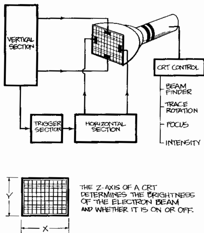
Figure 3. THE DISPLAY SYSTEM of your scope consists of the cathode-ray tube and its controls. To draw the graph of your measurements, the vertical system of the scope supplies the Y, or vertical, coordinates and the horizontal system supplies the X coordinates. There is also a Z dimension in a scope, it determines whether or not the electron beam is turned on, and how bright it is when it's on.
