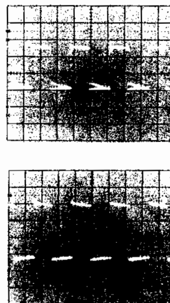
Figure 28. DIFFERENTIAL MEASUREMENTS allow you to remove unwanted information from a signal anytime you have another signal that closely resembles the unwanted components. For example, the first photo shows a 1 kHz square wave contaminated by a 60 Hz sine wave. Once the common-mode component (the sine wave) is input to channel 2 and that channel is inverted, the signals can be added with the ADD vertical mode. The result is shown in the second photo.
