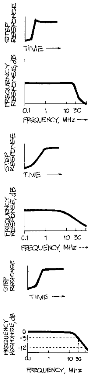
Figure 32. HIGH FREQUENCY COMPENSATION in a scope's vertical ampifier has an effect on the rise time of square waves measured by the scope. If too much high frequency compensation is present, the rise times will show overshoot and possible ringing, as in the top drawing. Too little, as shown in the second drawing, tends to roll off the edges of the square wave. A critically damped frequency response is best as in the third drawing.
