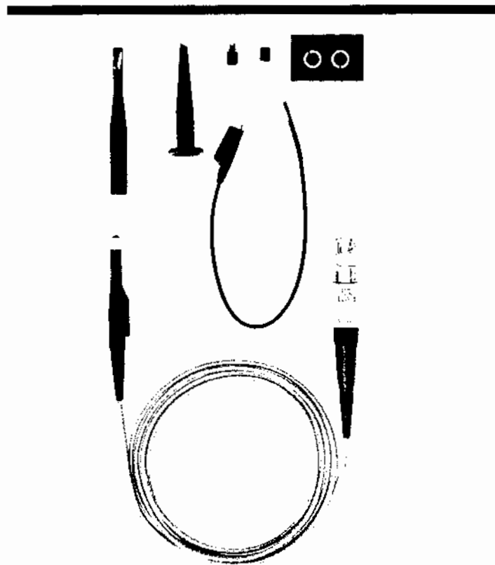
Figure 14. PROBES CONNECT THE SCOPE AND THE CIRCUIT-UNDER-TEST. Tektronix probes consist of a patented resistive cable and a grounded shield. Two P6122 probes and the accessories pictured above are supplied with every 2200 Series scope. The probe is a high impedance, minimum loading 10X passive probe. The accessories for each probe (from left to right) are: a grabber tip for ICs and small diameter leads, a retractable hook tip, and IC tester tip cover, an insulating ground cover, marker bands; and (in the center) the ground lead.
