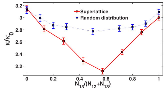
FIG. 4. (Color online) Thermal conductivity as a function of the ^{13}\text{C} concentration for superlattice (solid line) and random (dashed line) isotope distributions.
