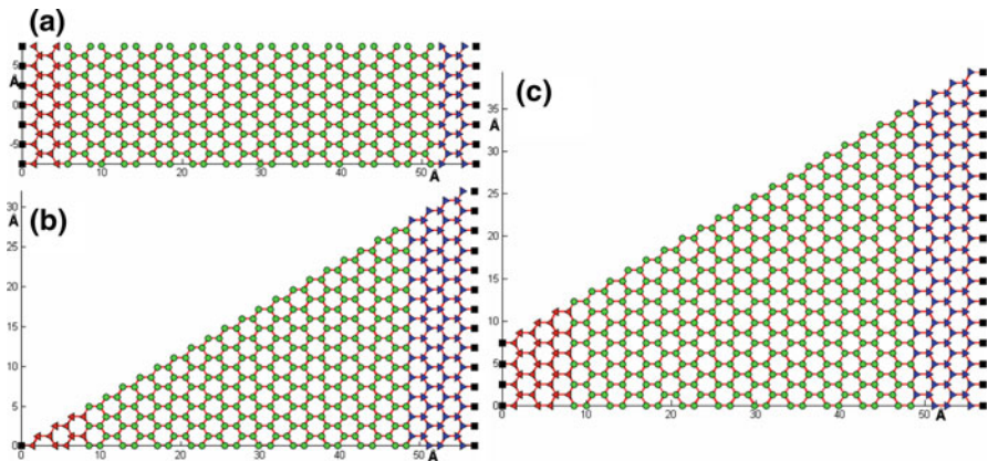
Fig. 1 Structures of GNRs in this study: (a) rectangle , (b) triangle , and (c) trapezoid
