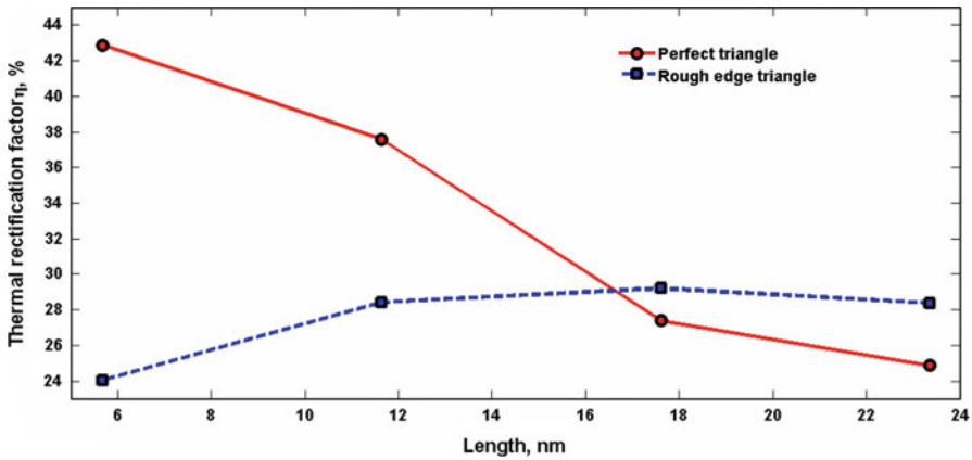
Fig. 4 Size dependence of TR factor for perfect and roughged edge triangular GNRs
