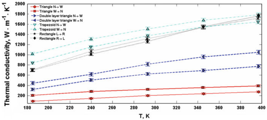
Fig. 2 TR of GNRs. The shape and size of the GNRs are specified in Fig. 1
