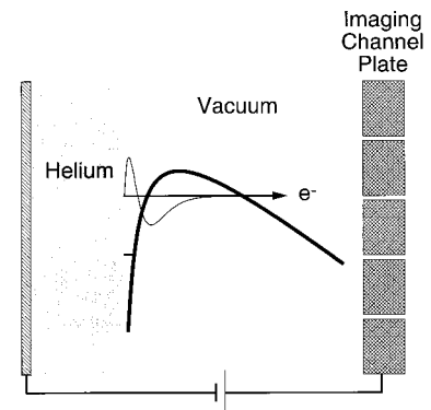
Fig. 3. The read-out configuration. The potential leading to tunneling when a reverse field is shown, along with a schematic of the position-sensitive channel plate.
