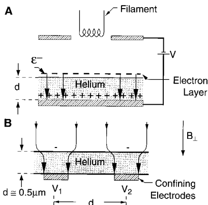
Fig. 2. (A) The parallel plate capacitor arrangement for confining a uniform layer of electrons. The holding field \mathcal{E}_{\perp} and the filament for charging are shown. (B) The geometry for a pair of electrons on a patterned substrate. The rough dimensions, the shape of the field lines, and the control gate are included.
