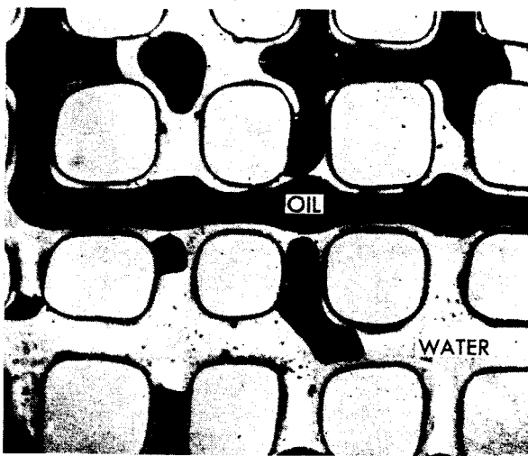
FLUID DISTRIBUTION in a slightly water-wet micromodel. Fig. 9.
