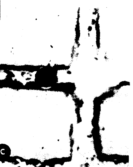
FILAMENT FLOW of oil in a slightly water-wet micromodel. Fig. 12.
