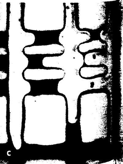
GROWTH OF WATER SLUGS in a strongly water-wet system. Fig. 11.
