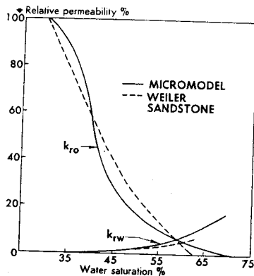
RELATIVE-PERMEABILITY curves from studies of a capillary micromodel and a natural sandstone. Fig. 5.
