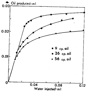
WATER-FLOOD behavior of the capillary micromodel. Fig. 3.
