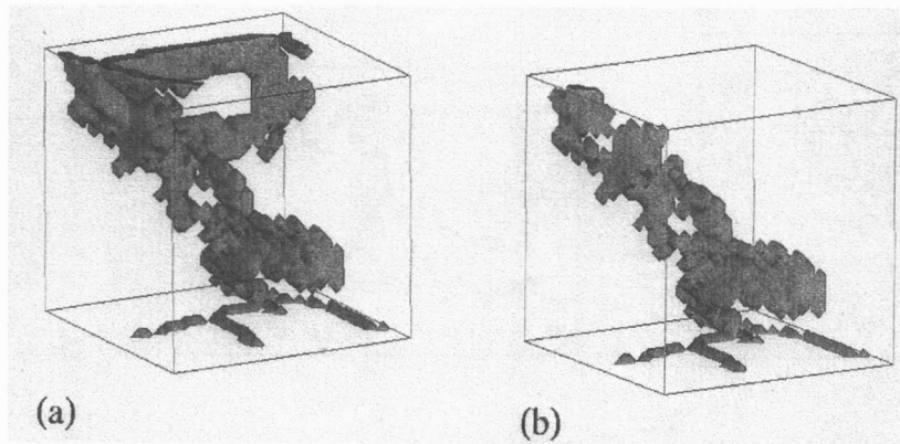
Figure 3. Three-dimensional visualization of the non-wetting phase flows in a subvolume of the natural fracture network in Core BB. (a) Fully invaded; (b) At breakthrough.
