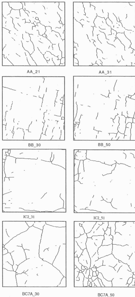
Figure 1. Two-dimensional images (60 mm by 60 mm) of fracture network for different depths within the coal cores from CT scans that were processed to remove beam hardening effects. The sample name is followed by the depth of the slice in mm.
