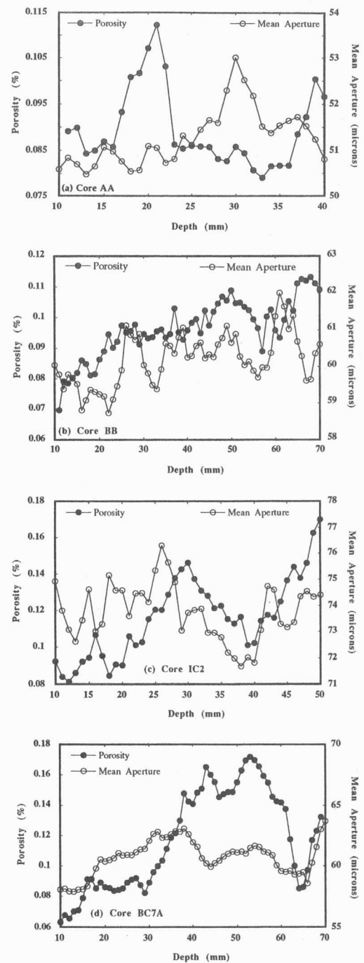
Figure 2. The variation in the porosity and mean aperture of the fracture network with depth in the sample for coal cores (a) AA, (b) BB, (c) IC2, and (d) BC7A.
