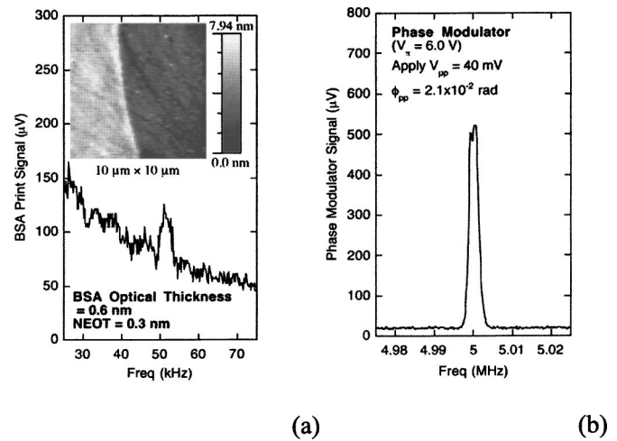
FIG. 2. The AO-BioCD calibration. (a) The homodyne signal spectrum of printed BSA. Insert: the atomic force microscope scan of the edge of one BSA spoke. (b) The homodyne signal spectrum of the phase modulator, driven by a 5 MHz ac voltage with V_{pp}=40 mV, which generates a phase modulation of \phi_{pp}=2.1 \times 10^{-2} rad for an equivalent optical thickness of 2.8 nm.
