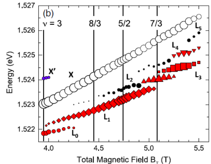
FIG. 2. (a) RRS results overlapped with optical emission for \nu = 2.50 from sample A. (b) Energy of the bands in the optical emission from sample A from the N = 1 LL as a function of total magnetic field B_T . The area of each data point is proportional to the integrated intensity found from a Lorentzian fit (except in the
