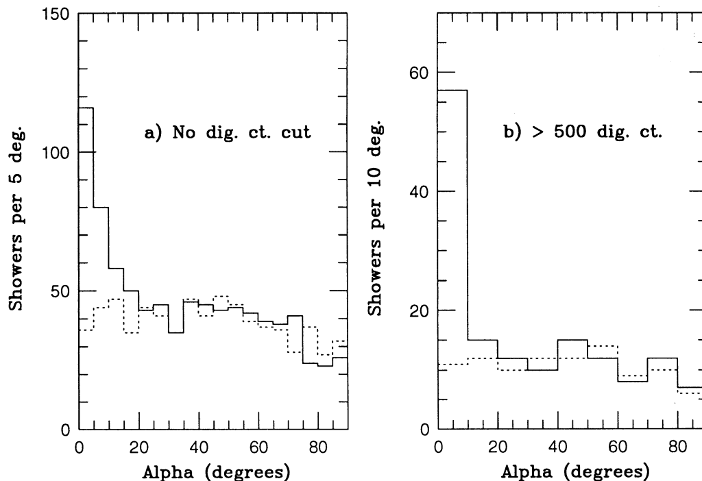
FIG. 1.—On- and off-source \alpha distributions for Mrk 421 for 1994 May 15.25 (UT). The distributions are for those showers for which the other supercuts selection criteria have been satisfied. The duration of each observation is 28.3 minutes. (a) No selection has been made on the number of digital counts contained in a shower image. (b) Only those showers which have more than 500 digital counts are retained. The latter selection is approximately equivalent to raising the threshold energy from 250 to 500 GeV.
