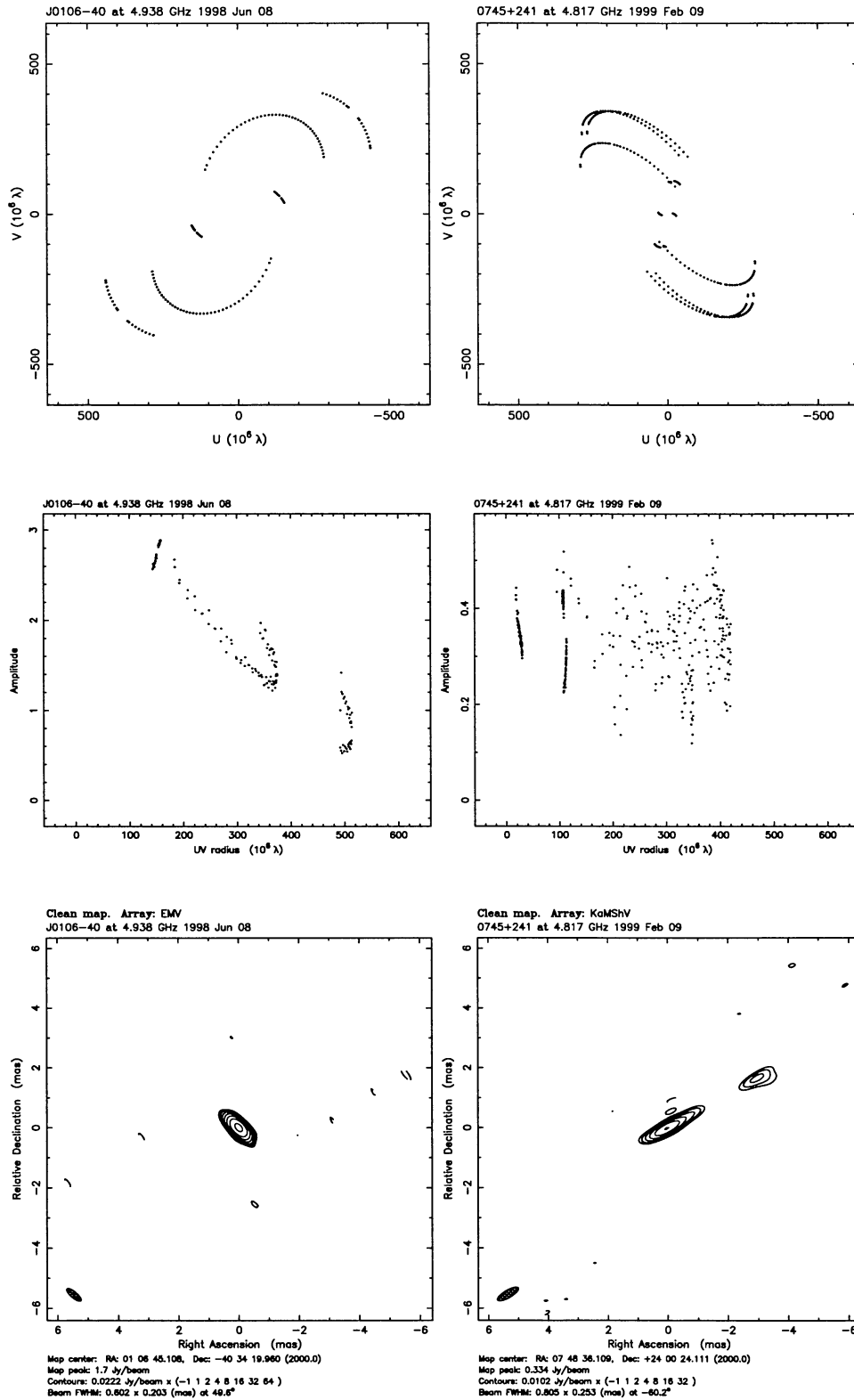
Fig. 1. Typical results for two survey sources: (Top) the (u, v) coverages; (Middle) the visibility plots; (Bottom) the images. The left panel is for survey source J0106-40 at epoch 1998.43. The ground telescopes were Hobart and Hartebeesthoek, the tracking station was Madrid, the correlator was Penticton, and the on-source time was 6.3 hr. The right panel is for survey source 0745+241 at epoch 1999.11. The ground telescopes used were Kashima, Mopra and Shanghai, the tracking station was Usuda, the correlator was Mitaka, and the total on-source time was 5.3 hr.
