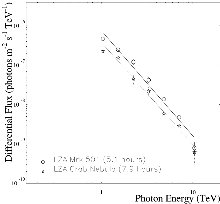
FIG. 5.—Energy spectrum of Markarian 501 (LZA data only) in comparison to the spectrum of the Crab Nebula derived with the same method. A power-law fit to the Markarian 501 data gives a \chi^2 = 14.7 for 5 d.o.f. (probability of 0.015).
