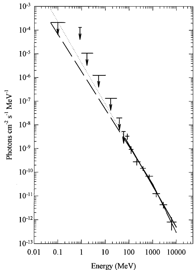
FIG. 3.—Phase-averaged gamma-ray energy spectrum of PSR B1055–52. The fits in the energy range 70 MeV–10000 MeV to a power law and a power law with a break at 1000 MeV are described in the text, with extrapolations to lower energies shown as dotted and dashed lines respectively. The uncertainties shown are statistical only.
