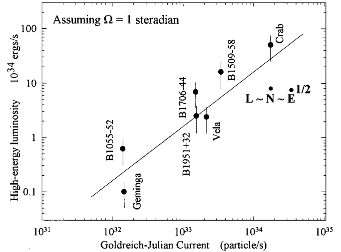
FIG. 5.—Pulsar luminosities, integrated over photon energies above 1 eV, assuming radiation into one sr, vs, Goldreich-Julian current \dot{N} \sim \dot{E}^{1/2} .
