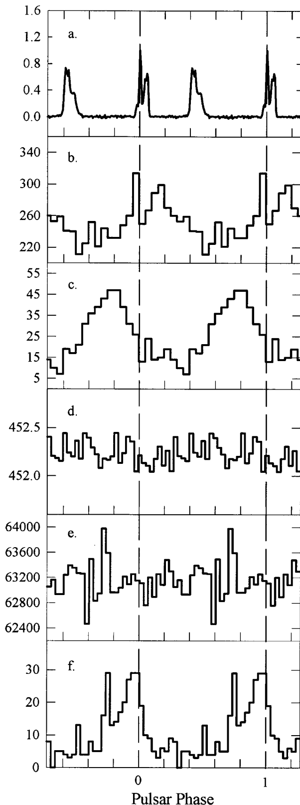
FIG. 2.—Multiwavelength light curves for PSR B1055–52. The spectral band and intensity units are as follows: (a) radio, 1520 MHz, relative intensity; (b) ROSAT X-rays less than 0.5 keV (Ögelman & Finley 1993); (c) ROSAT X-rays greater than 0.5 keV (Ögelman & Finley 1993); (d) OSSE gamma rays, 48–184 keV photons \text{s}^{-1}\text{ detector}^{-1} ; (e) COMPTEL gamma rays 0.75–30 MeV; (f) EGRET gamma rays > 240\text{ MeV} . Two complete cycles are shown. The radio reference is shown by a vertical dashed line.
