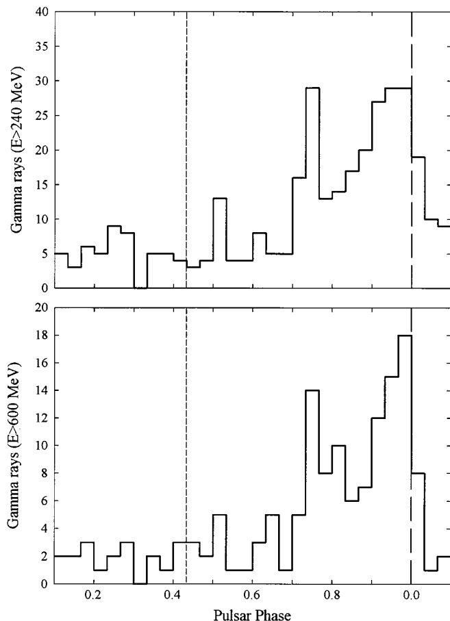
FIG. 1.—High-energy gamma-ray light curve for PSR B1055–52. The 197 ms period is divided into 30 phase bins. The double radio pulse has peaks with centroids at phases 0.43 ( short-dashed vertical line ) and 0.0 ( long-dashed vertical line ). Top : gamma rays above 240 MeV selected from a fixed cone with radius 1^\circ 7' ; bottom : gamma rays above 600 MeV selected from an energy-dependent cone, as described in the text.
