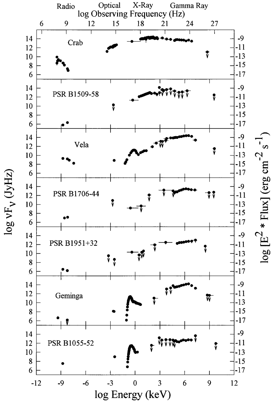
FIG. 4.—Multiwavelength energy spectra for the known gamma-ray pulsars. References for this figure are given in Table 3.
