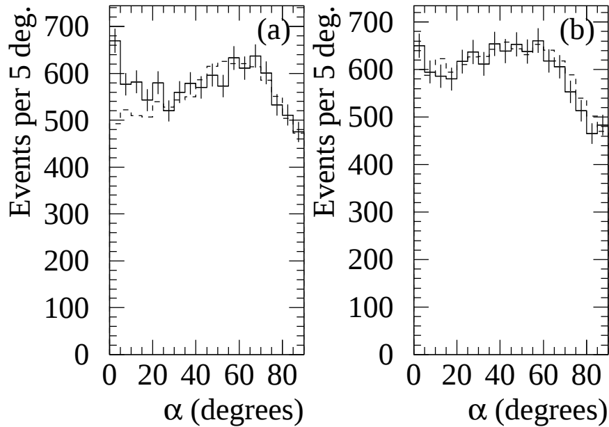
FIG. 2.—Distributions of the \alpha parameter for 1ES 2344+514 for events that pass all other Supercuts95 cuts. Shown are all on-source data taken in (a) 1995/96 and (b) 1996/97. The dashed curves are the \alpha distributions for the nonsource runs used in each season to estimate a tracking ratio (see text for details) normalized to the predicted background in the \alpha = 0^\circ – 15^\circ region.
