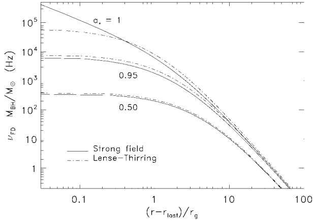
FIG. 1.—Disk precession frequency (multiplied by black hole mass), as a function of distance from the last stable orbit, for various black hole angular momentum (assuming that Q = 0.01 ; see text). The weak-field limits are also shown in dash-dotted lines for comparison.
