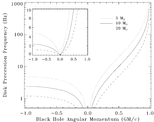
FIG. 2.—Disk precession frequency where the disk emission peaks ( r_{\text{peak}} ), as a function of the dimensionless specific angular momentum ( a_* ) of Kerr black holes (assuming that Q = 0.01 ).
