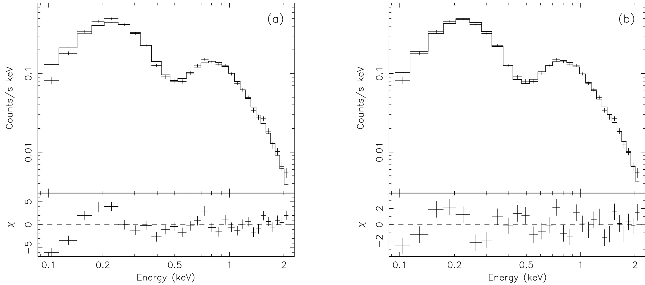
FIG. 3.—X-ray spectrum of the nuclear source. The solid-line histograms represent the best-fit models to the data: (a) PL + RS and (b) PL + RS + GAU.
