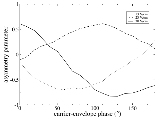
FIG. 4. Dependence of the ejection direction on the carrier-envelope phase. Shown is the ejection asymmetry parameter for RF amplitudes of 13 V/cm (dashed line), 23 V/cm (dotted line), and 30 V/cm (solid line). A value of zero means symmetric ejection in both directions. The Rydberg population is depleted for amplitudes \geq 18 V/cm. The 6 MHz pulses are 300 ns long.
