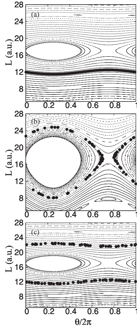
FIG. 2. Classical phase-space structure for the one-dimensional rigid rotor driven from L = 12 to 22 at the 10-photon resonance with a peak intensity of I_0 = 1.8 \times 10^{11} W/cm 2 seen in the lower panel of Fig. 1. Panels (a) and (c) are snapshots in time during the rising and falling edges of the Gaussian pulse envelope at intensities 2.26 \times 10^{10} W/cm 2 and the middle panel is at the peak of the pulse. Larger points mark the phase-space coordinates of the classical trajectories, initially loaded onto the L = 12 line as seen in (a). As the field intensity is increased, the island created at the driving frequency grows larger and eventually touches the L = 12 line, resulting in transportation of the trajectories on the L = 12 line to above the island. As the field is decreased back down, substantial fraction of the population ends up in L = 22 as seen in (c).
