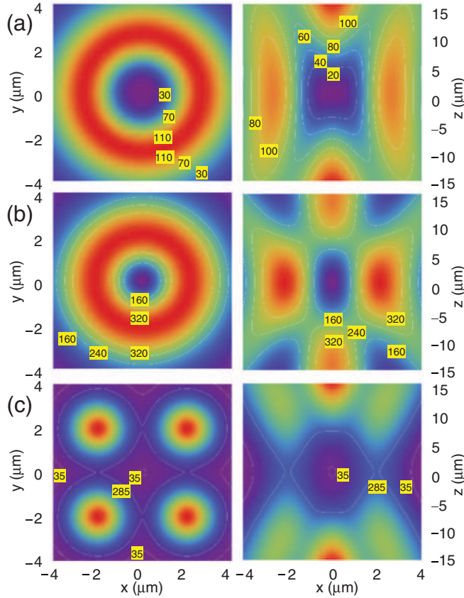
FIG. 3. (Color online) Trapping depth of blue-detuned dipole traps in the x - y (left column) and x - z (right column) planes for Cs 6s , \lambda = 780 nm, \alpha = -235 \times 10^{-24} cm ^3 , power P = 50 mW for (a) Gaussian interference BBT, w_1 = 2 \mu m and w_2 = 3.78 \mu m; (b) crossed vortex BBT, w = 3 \mu m and \theta = 8.6^\circ ; and (c) Gaussian lattice trap, w = 1.5 \mu m and d = 4 \mu m.
