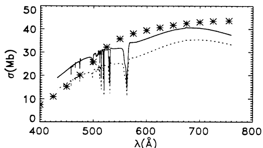
FIG. 1. Experimental and theoretical total photoionization cross section of Cl as a function of wavelength. *, experimental points of Ref. [4]; solid line, length gauge calculation; dotted line, velocity gauge calculation. The {}^3P^o thresholds are near 505 Å and the {}^1P^o thresholds are near 455 Å. The rest of the figures are plotted as a function of frequency with \omega (eV) \cong 12400/\lambda (Å).
