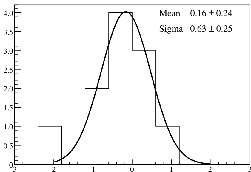
Figure 4. Pull distribution comparing the fit results shown in table 1 to the neutrino mass that was assumed in the various simulation trials.
