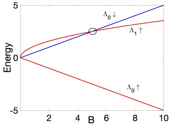
Figure 1. The schematic plot of the composite fermion \Lambda levels. When the in-plane magnetic field affecting Zeemann splitting of electrons as well as composite fermions, is increased, while the orbital out-of plane component of magnetic field keeps the system on the fractional quantum Hall plateau, there is a level crossing (black circle) of the \Lambda_{0\downarrow} and \Lambda_{1\uparrow} defining B^* , which leads to a spin transition from spin-unpolarized state to spin-polarized state.
